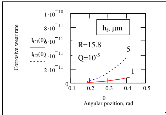
Figure 9. Corrosive wear rate versus impact angle
