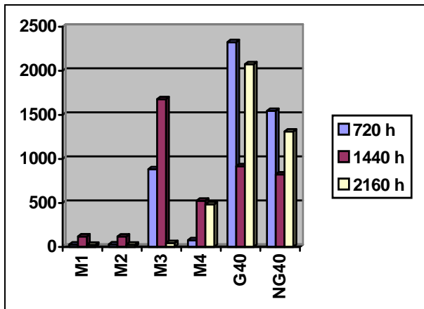
Figure 12. Corrosion rate of ball and seat materials
