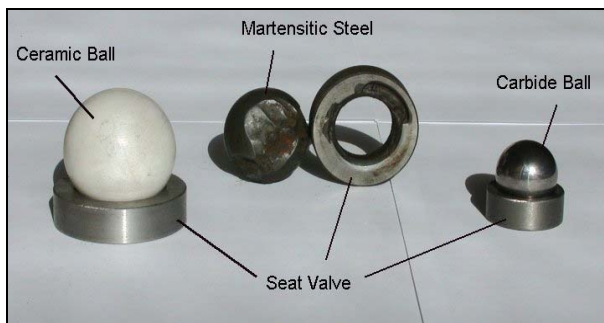
Figure 10. Picture of ball
