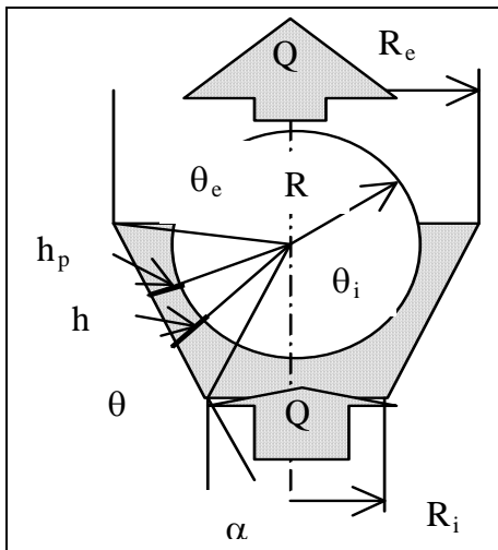
Figure 1. Geometry gape for the flow model of crude petroleum liquid.
