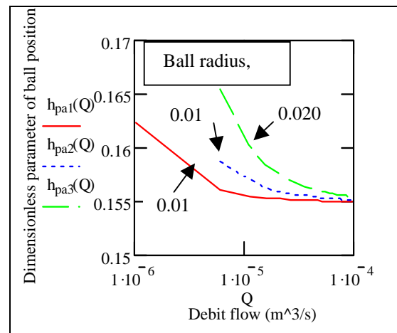
Figure 2. Position ball in conical gape
