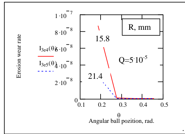
Figure 8. Erosion wear rate vs. angular ball position and ball radius
