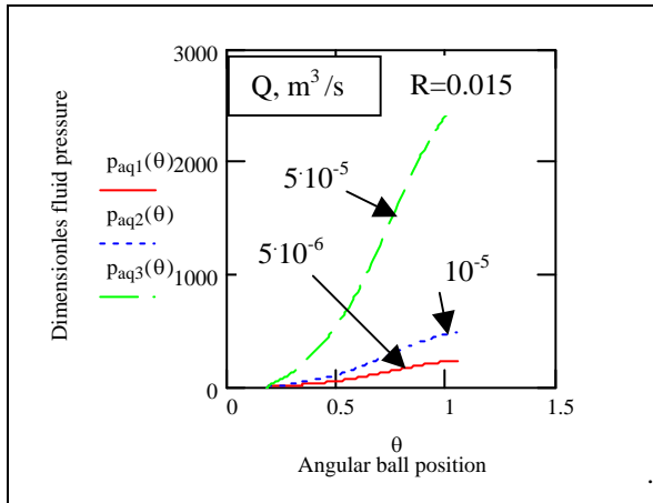
Figure 4. Fluid pressure in gap for diverse flow rates
