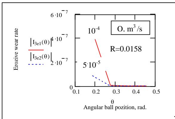
Figure 7. Erosion wear rate vs. angular ball position
