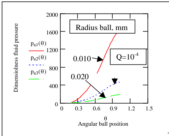
Figure 4. Fluid pressure in gap
