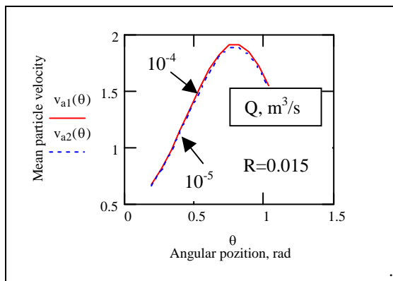
Figure 5. Mean particle velocity in gap
