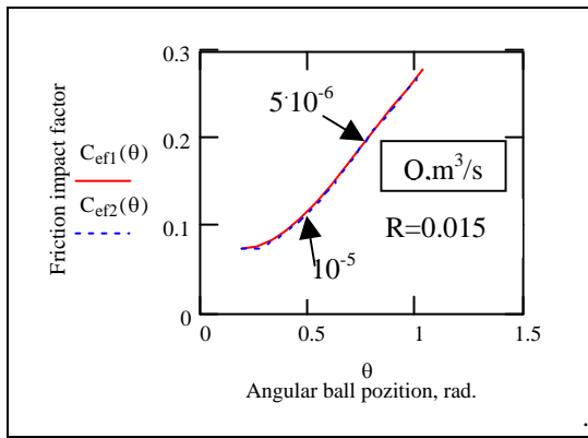
Figure 6. Friction impact factor for ball
