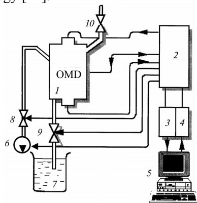
Figure 3. In-line wear monitoring optomagnetic detector: 1 – sensor; 2 – electronic unit; 3 – ADC; 4 – input/output unit; 5 – PC; 6 – pump; 7 – oil tank; 8, 9, 10 – electromagnetic valves
