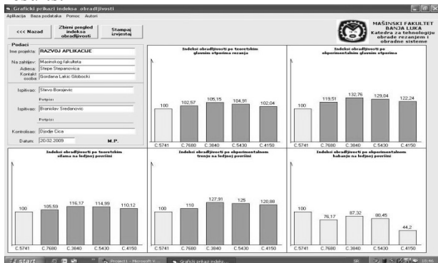
Figure 5. Histogram of machinability index for the group of tough materials
