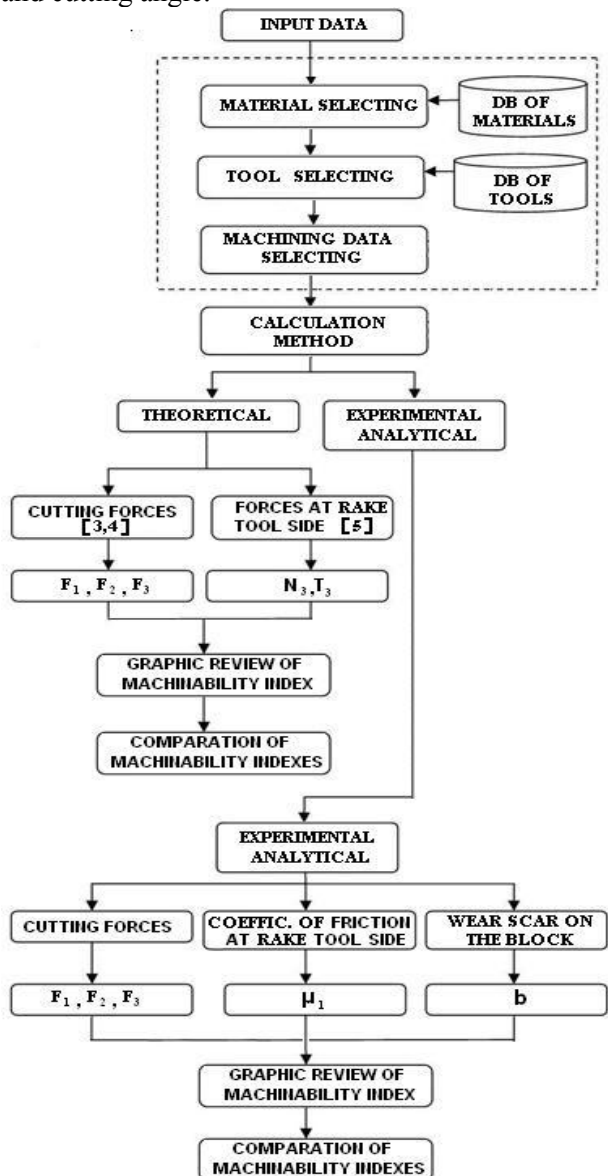
Figure 3. Flow-chart of application for machinability index calculation
