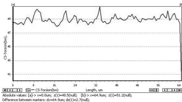
Figure 6. Rotational deflection of the AFM cantilever of enamel under dry condition
