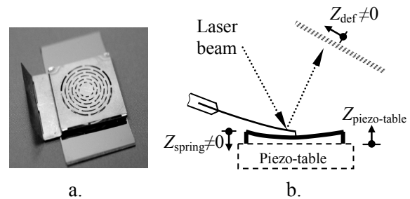
Figure 4. Measurement of the stiffness of the cantilever with spherical tip by use a microspring:
