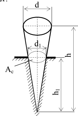
Figure 5. Contact area A_c gives by the indentation of sample with an AFM conical cantilever
