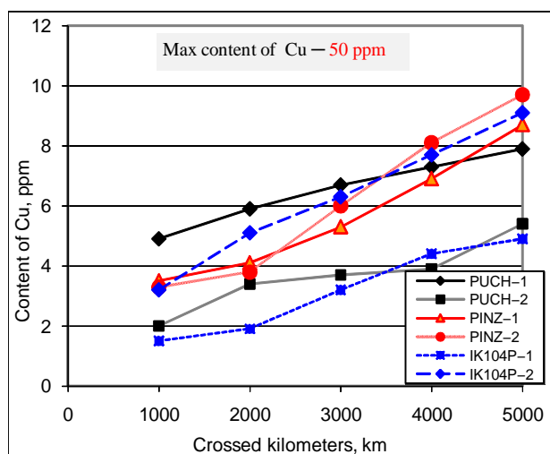
Fig. 7. The change of content Cu [10].
