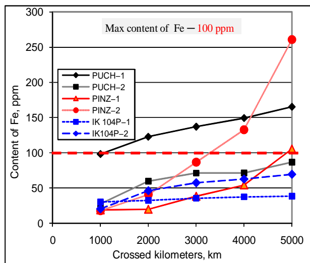
Fig. 6. The change of content Fe [10].
