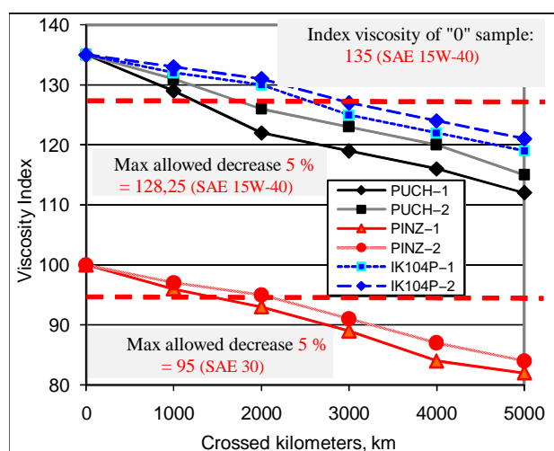
Fig. 1. The change of Viscosity Index [10].
