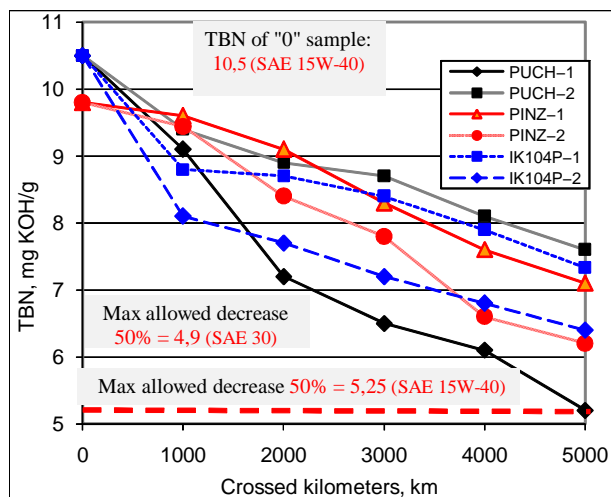
Fig. 4. The change of TBN [10].
