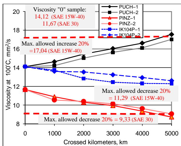
Fig. 3. The change of viscosity at 100°C [10].
