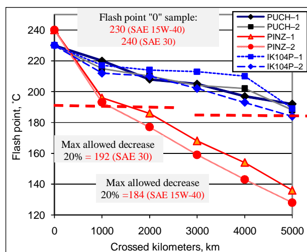
Fig. 5. The change of flash point [10].
