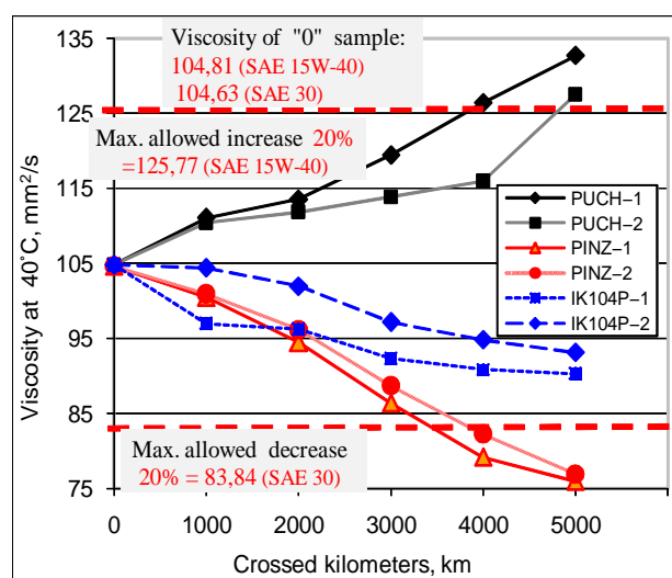
Fig. 2. The change of viscosity at 40 °C [10].
