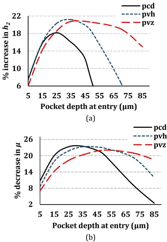
Fig. 6. Variation of performance behaviours (a) enhancement in film thickness (b) decrease in friction coefficient for different pocketed pads with reference to plain pad [unit load = 5 MPa, \theta_p/\theta_o=0.7 ].
