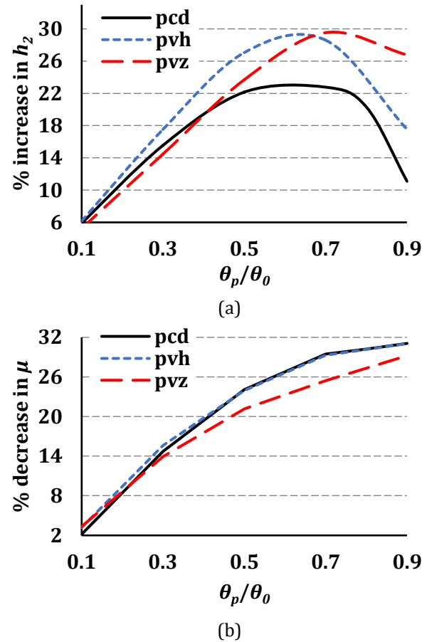
Fig. 8. Variation of performance behaviours (a) increase in film thickness (b) decrease in \mu for different pocketed pads with reference to plain conventional pad [unit load =2 MPa, d_{pi}=40 \mu\text{m} ].
