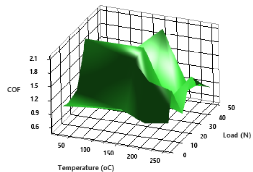
Fig. 7. COF surface plot as a function of load and temperature.
