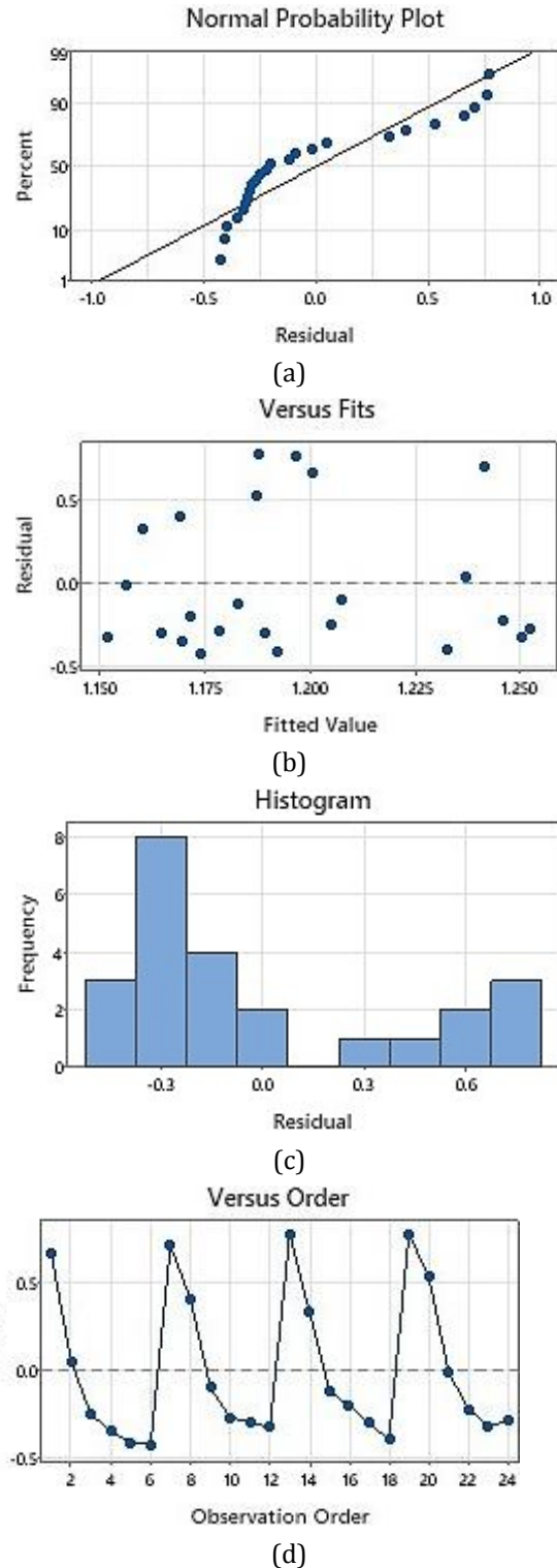
Fig. 5. Residuals plots for COF (a) Normal probability plot, (b) Versus fits, (c) Histogram, (d) Versus order.
