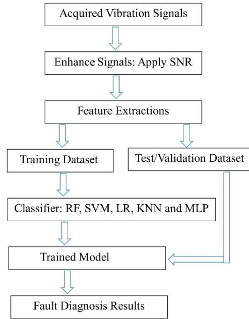
Fig. 3. Flow chart of fault diagnosis models.
