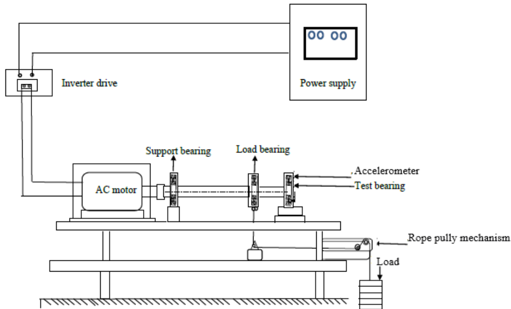
Fig. 2. Schematic diagram of experimental test rig.
