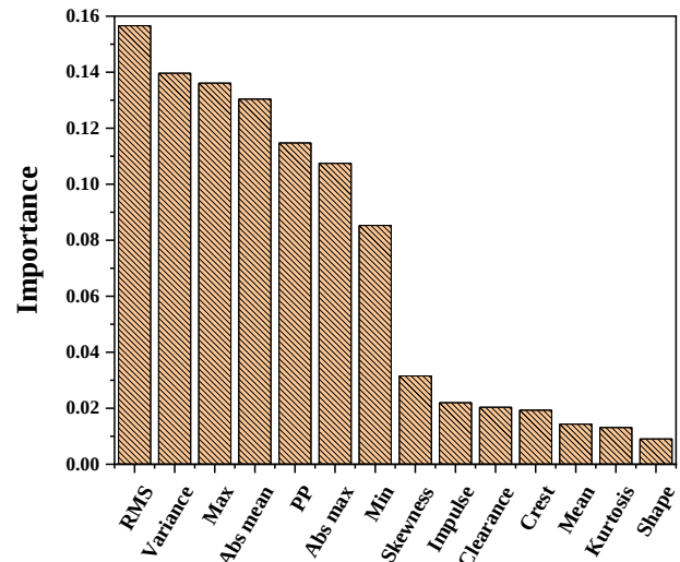
Fig. 6. Feature mapping.
