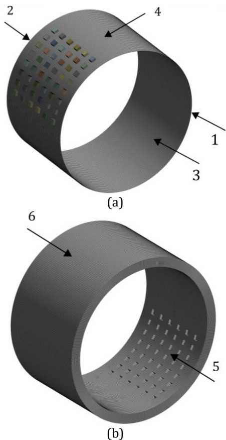
Fig. 2. Mesh configurations for lubricant and bearing with boundary conditions: (a) lubricant mesh; (b) bearing mesh.
