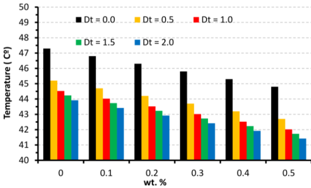
Fig. 15. Variations in temperature against the Dt and Wt. of TiO 2 nanoparticles at \varepsilon = 0.3 in the pressure-increasing region.
