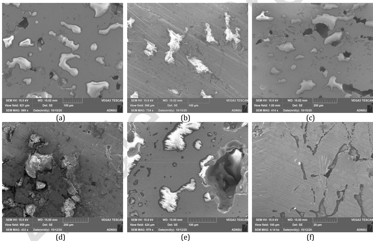
Fig. 8. Deformation of glass particles during sintering at compaction pressures of: (a, b) 400 MPa; (c, d) 800 MPa; and (e, f) 1000 MPa. The cast iron and glass contents were 30 and 6 wt.%, respectively, in (a, c, e), and 40 and 8 wt.%, respectively, in (b, d, f).
