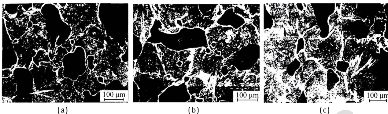
Fig. 6. Microstructure of the Fe-CI-Glass powder composite material oxidized at 200 °C: a), b), c) – oxidation duration of 1, 2, and 3 hours, respectively.
